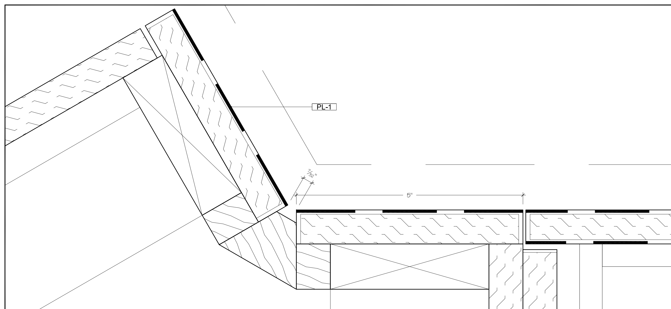
9 SECTION DETAILS SCALE: FULL CORNER REVEAL CIRCULATION 103
