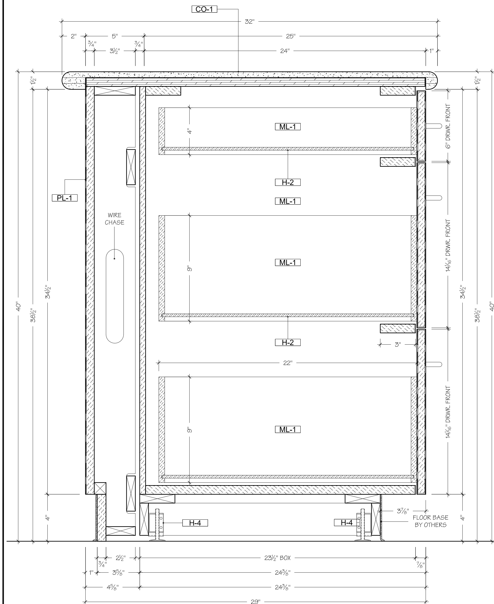
4 SECTION CIRCULATIONDESK SCALE: 3" = 1'- 0" CIRCULATION 103
