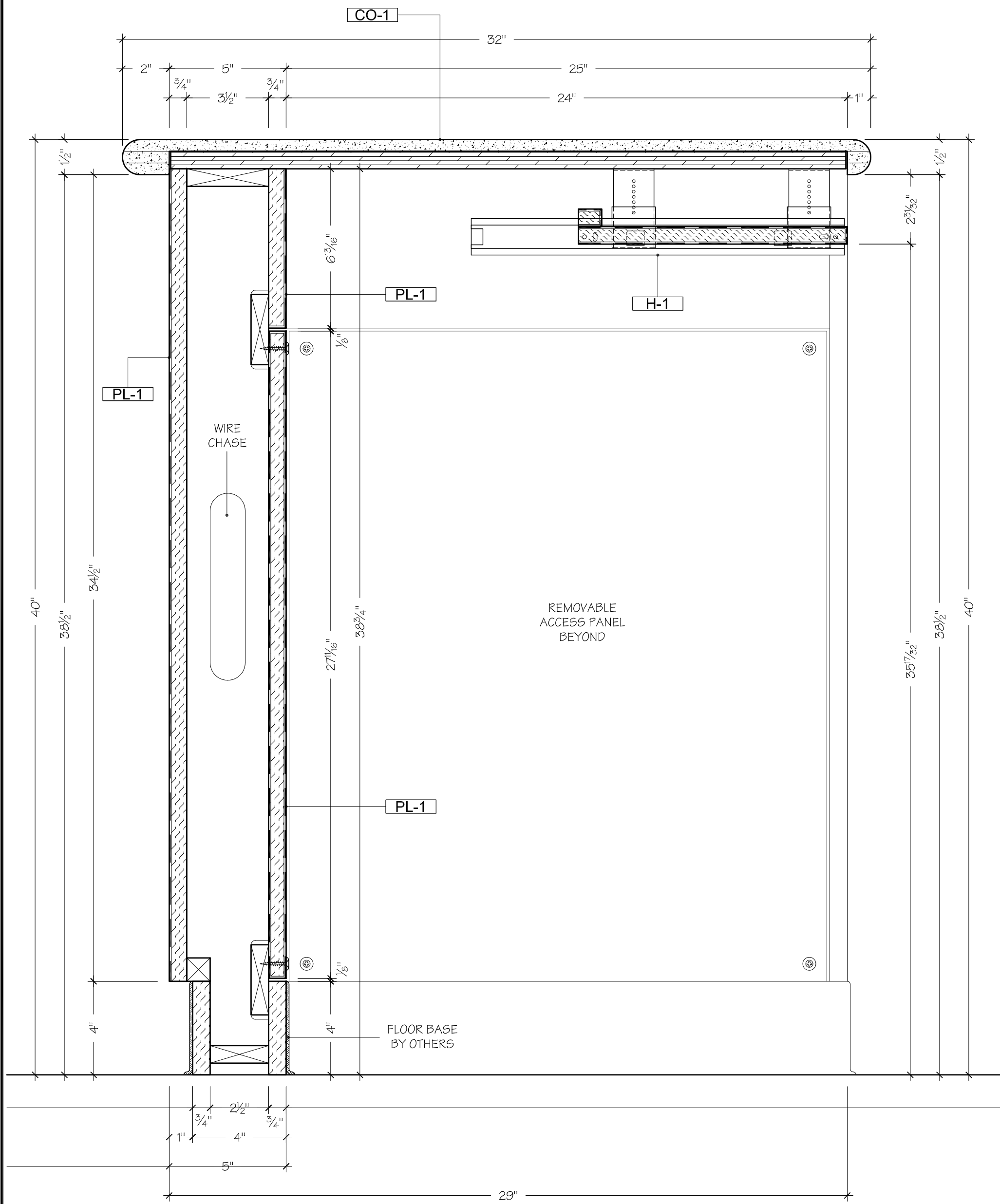
1 SECTION SCALE: 3" = 1'-0" CIRCULATIONDESK CIRCULATION 103
