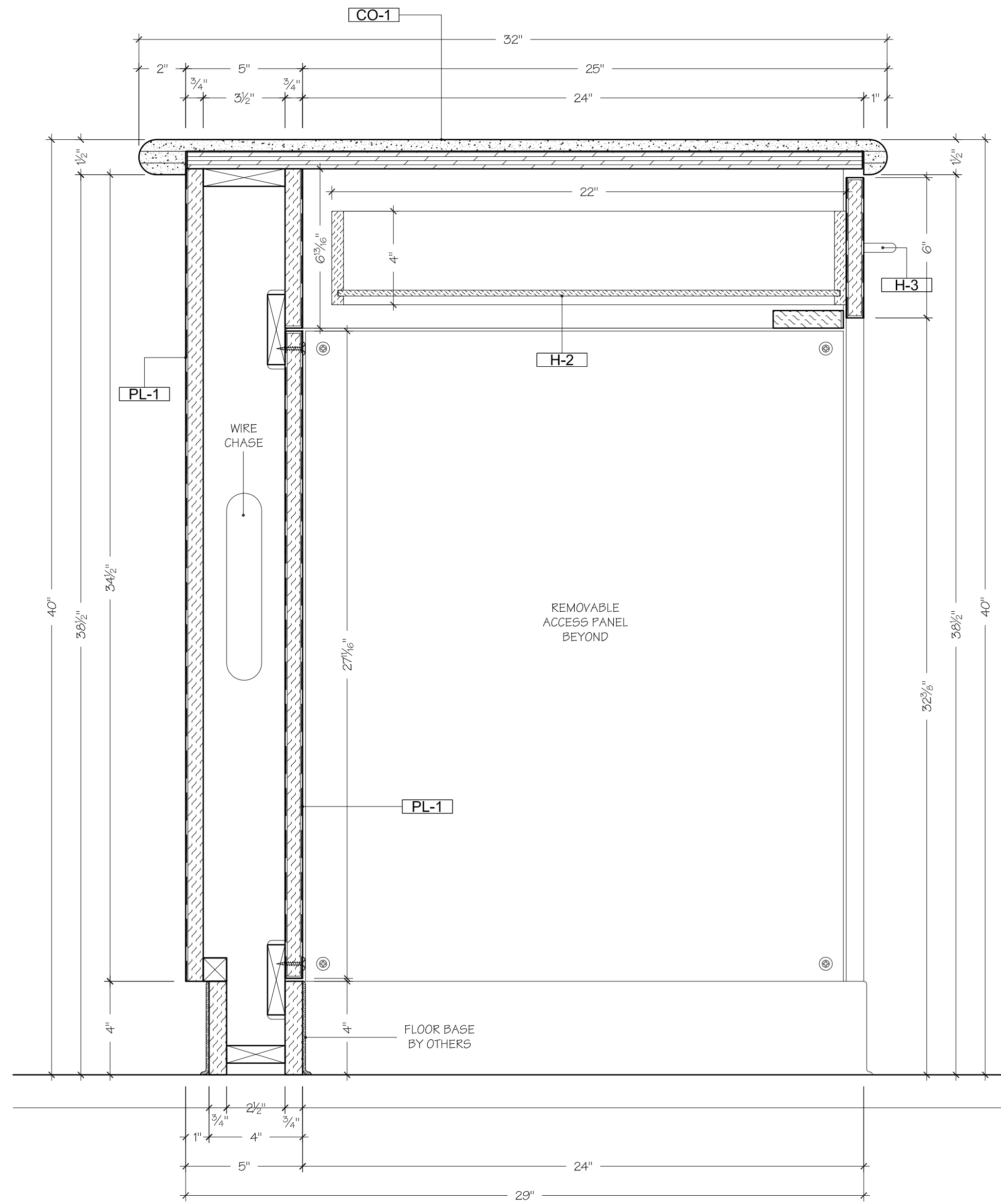
2 SECTION SCALE: 3" = 1'-0" CIRCULATIONDESK CIRCULATION 103
