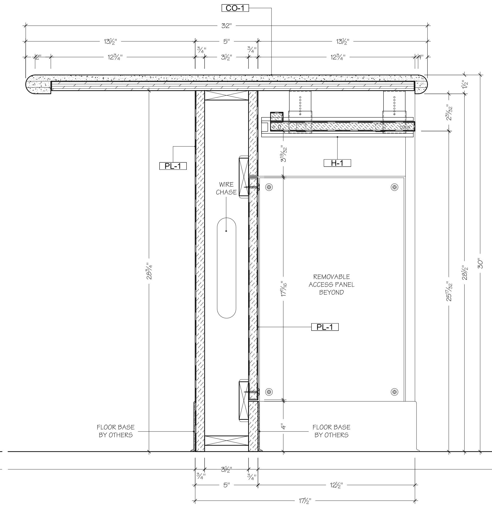
3 SECTION SCALE: 3" = 1'-0" CIRCULATIONDESK CIRCULATION 103
