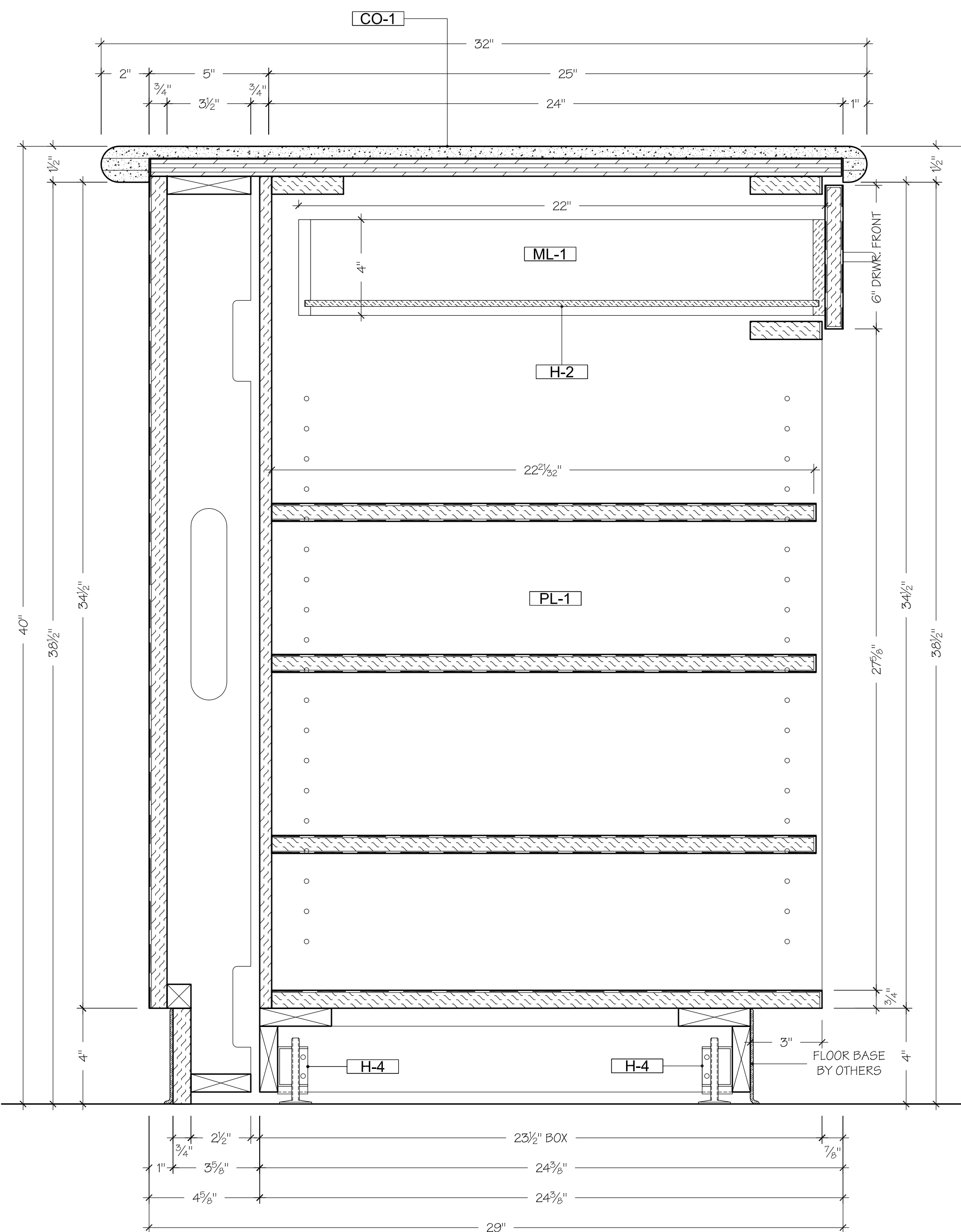
5 SECTION CIRCULATIONDESK SCALE: 3" = 1'- 0" CIRCULATION 103
