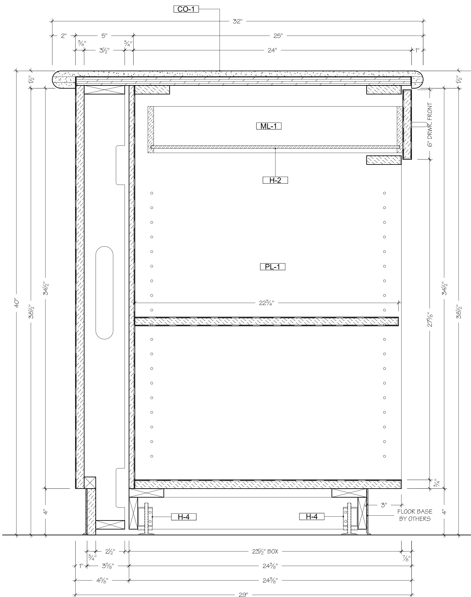
6 SECTION CIRCULATIONDESK SCALE: 3" = 1'- 0" CIRCULATION 103
